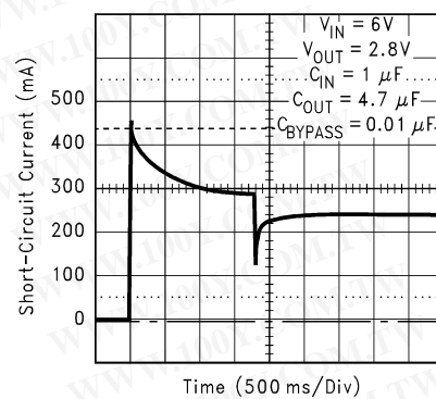
Short-Circuit Current
