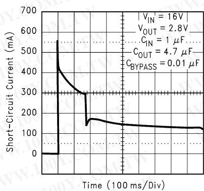
Short-Circuit Current
