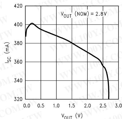
Short Circuit Current vs Output Voltage
