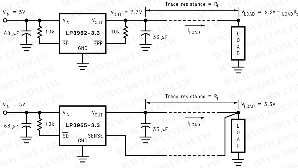
FIGURE 2. Improving remote load regulation using LP3965
