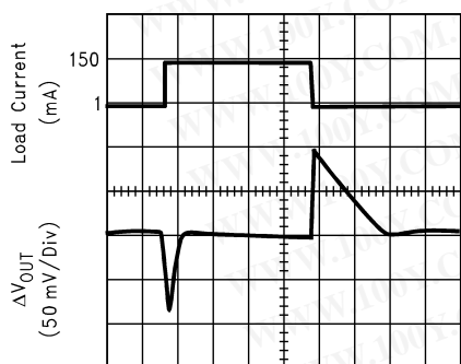
Load Transient Response ( V_{IN} = 3.2\text{V} )
