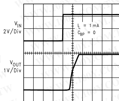
Start Up Time ( V_{IN} = 4.2\text{V} )
