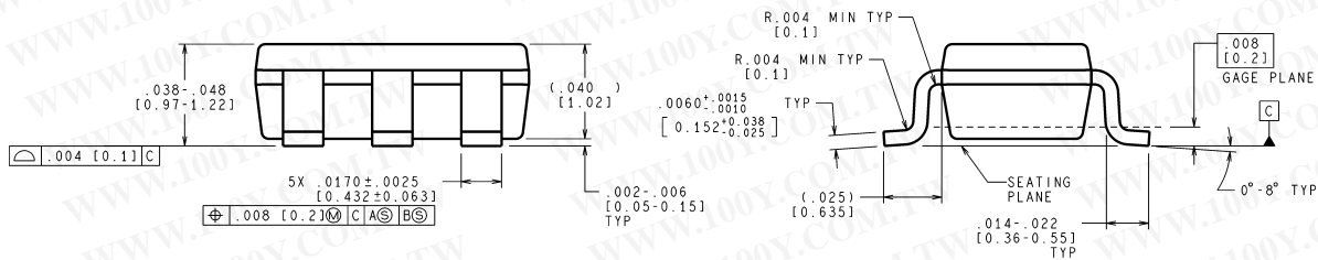
5-Lead Small Outline Package (MF) NS Package Number MF05A
