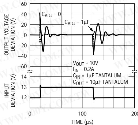
LT1084 Line Transient Response
