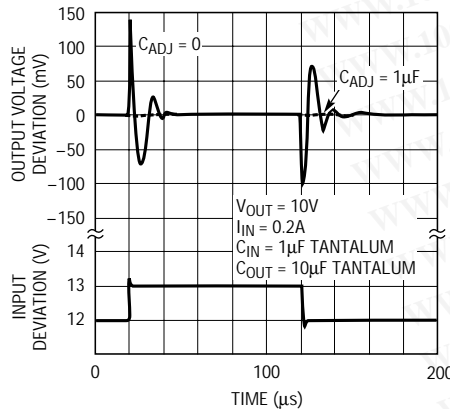
LT1083 Line Transient Response
