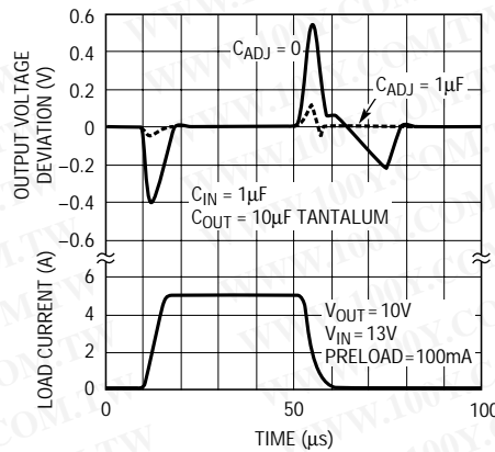
LT1084 Load Transient Response
