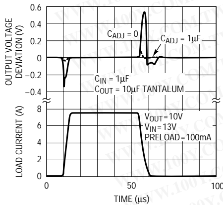
LT1083 Load Transient Response
