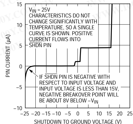
SHDN Pin Characteristics
