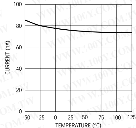
SENSE Bias Current (Adjustable Part)
