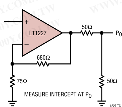
Test Circuit for 3rd Order Intercept
