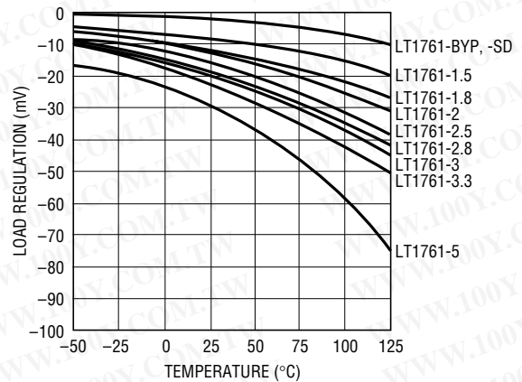
Load Regulation ΔI_L = 1mA to 100mA
