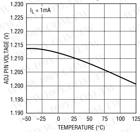
LT1963 ADJ Pin Voltage
