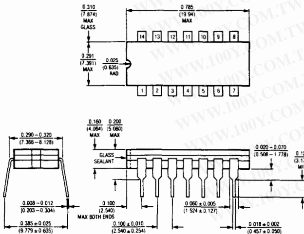
J Package 14-Lead Hermetic DIP
