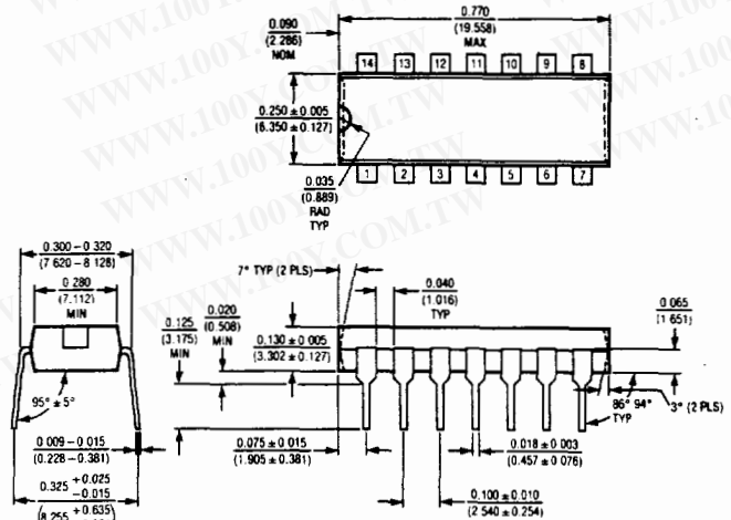
N Package 14-Lead Plastic
