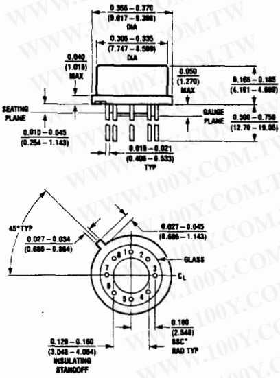
H Package Metal Can
