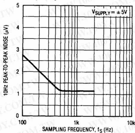
10Hzp-p Noise vs Sampling Frequency
