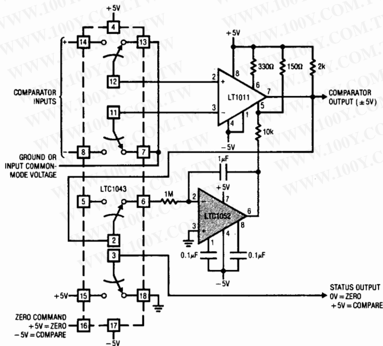
Offset Stabilized Comparator
