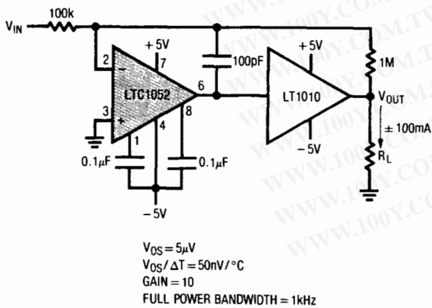
± 100mA Output Drive
