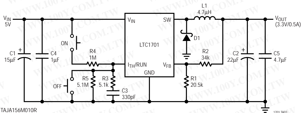
5V to 3.3V Converter with Push-Button On/Off
