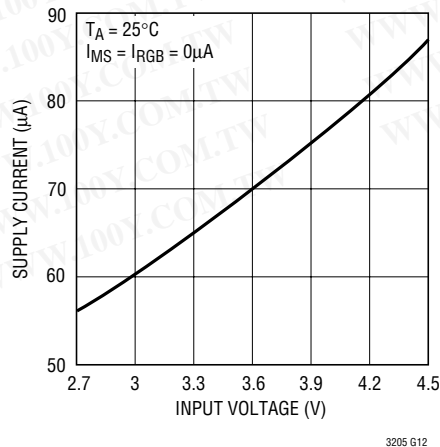
1:1 Mode No Load Supply Current vs VIN
