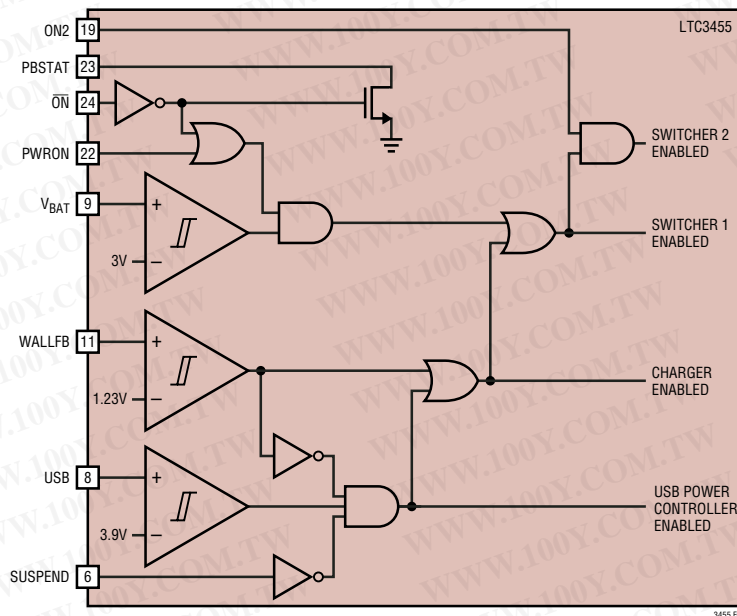
Figure 3. Turn-On Logic Diagram for LTC3455
