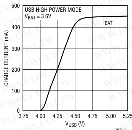
Figure 13. Charge Current vs USB Voltage
