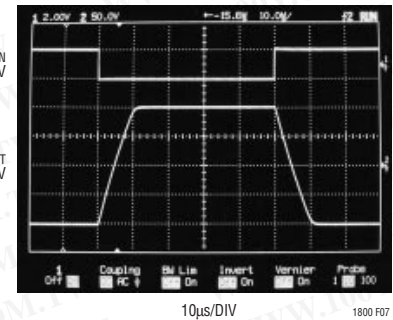
Figure 7. Large-Signal Time Domain Response of the Amplifier
