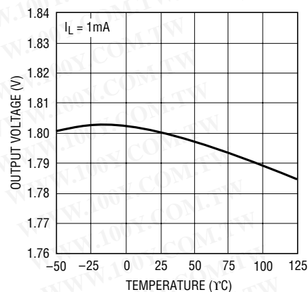
LT1963A-1.8 Output Voltage
