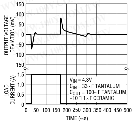
LT1963A-3.3 Transient Response
