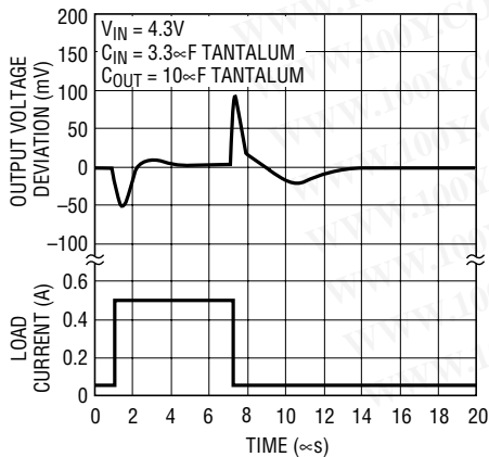
LT1963A-3.3 Transient Response
