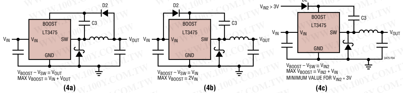
Figure 4. Generating the Boost Voltage
