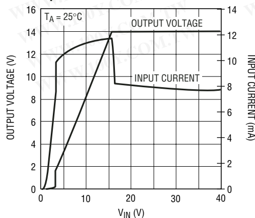
Open-Circuit Output Voltage and Input Current
