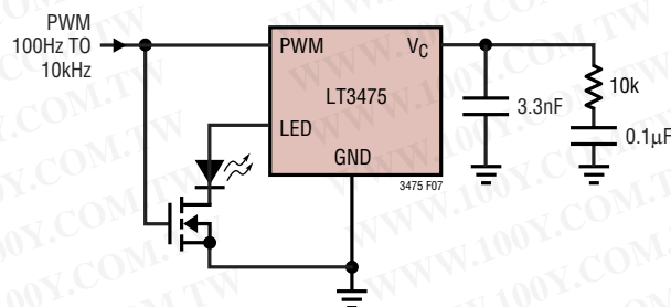
Figure 7. Dimming Using PWM Signal
