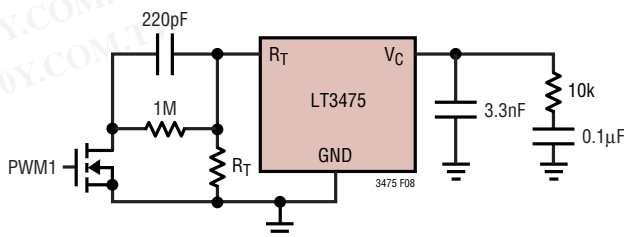
Figure 8. Extending the PWM Dimming Range
