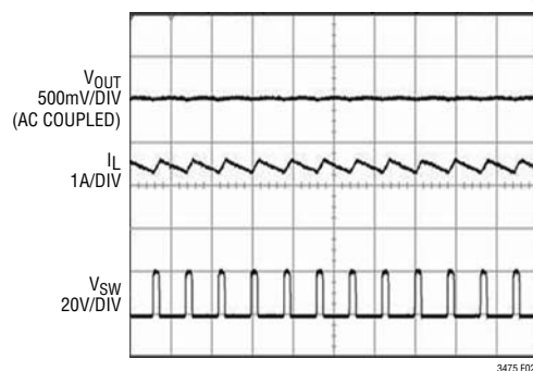
Figure 2. Operation at V_{IN(MAX)} = 20\text{V} . V_{OUT} = 3\text{V} and f_{SW} = 1.2\text{MHz}
