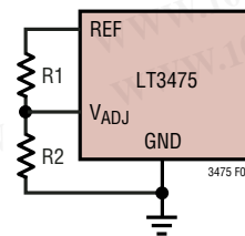
Figure 5. Setting V_{ADJ} with a Resistor Divider
