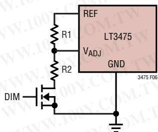
Figure 6. Dimming with a MOSFET and Resistor Divider
