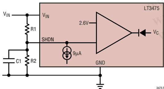
Figure 1. Undervoltage Lockout
