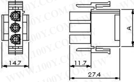
2, 3, 4 Circuit (In-Line)
