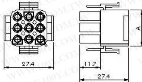
9, 12, 15 Circuit (Matrix)
