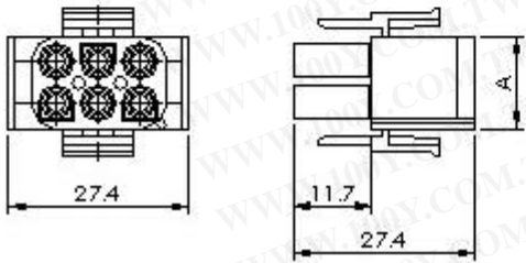
6 Circuit (Matrix)
