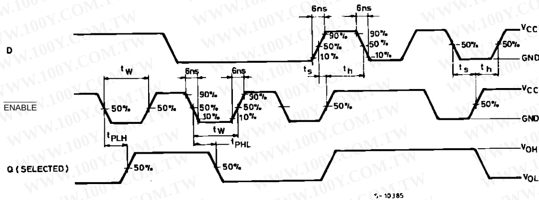
WAVEFORM 4. ( \text{D} = \text{H} , \text{A} \sim \text{C} = \text{Stable} )
