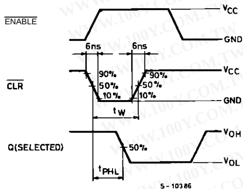
WAVEFORM 4. ( \text{D} = \text{H} , \text{A} \sim \text{C} = \text{Stable} )
