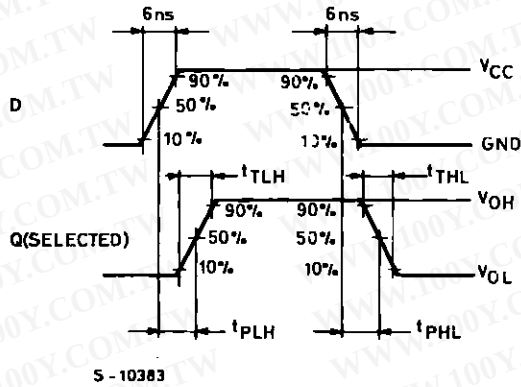
WAVEFORM 3. ( \overline{\text{CLR}} = \text{H} , \text{A} \sim \text{C} = \text{Stable} )
