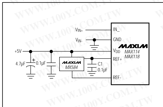
Figure 7b. External Reference, 4.096V Full Scale
