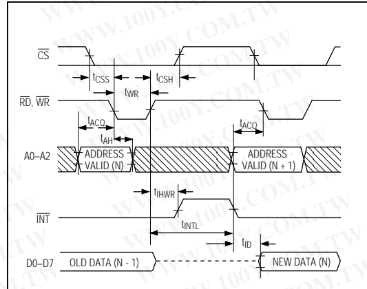
Figure 6. Pipelined Mode Timing (WR = RD) (MODE = 1)
