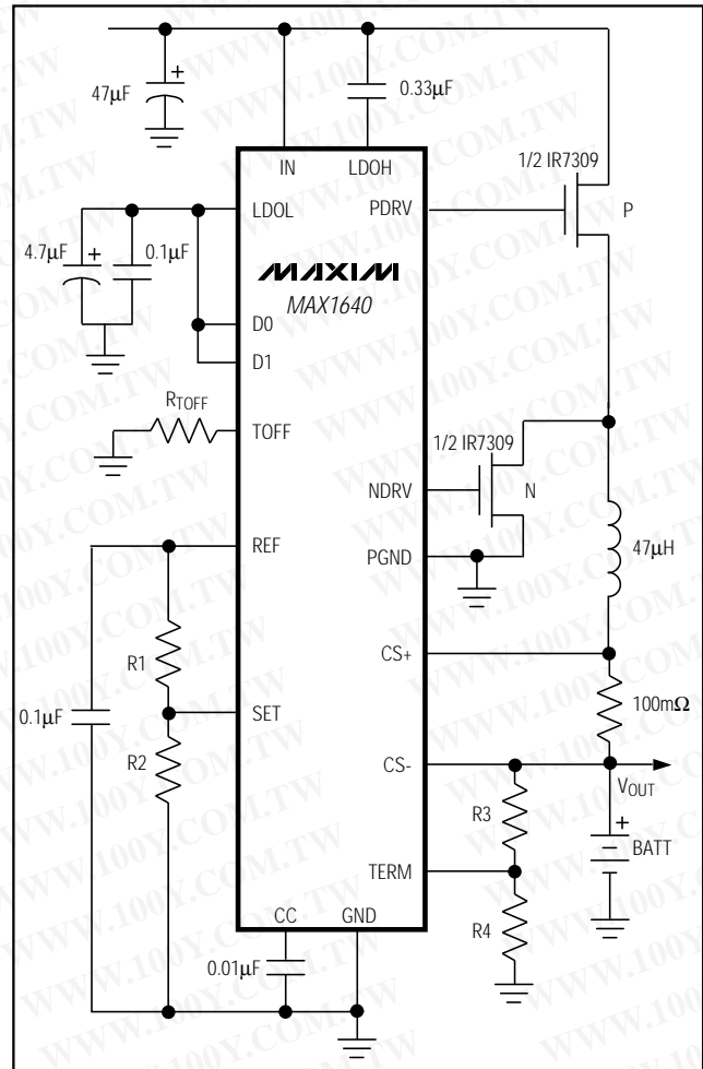
Figure 2b. Standard Application Circuit
