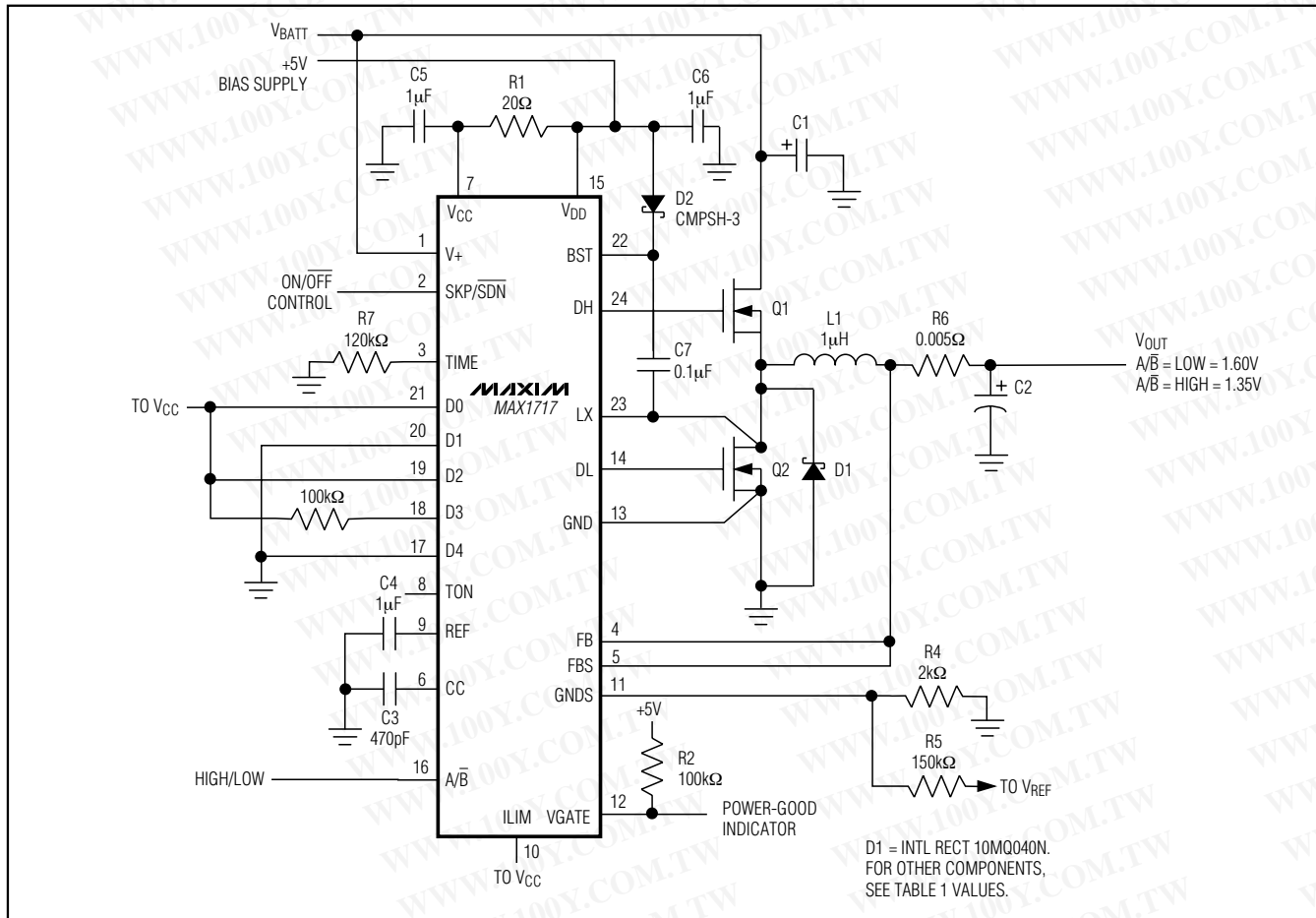
Figure 3. Voltage-Positioned Circuit
