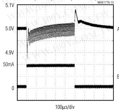
LOAD TRANSIENT (L = 10 \mu H , 500 \mu s PULSE)
