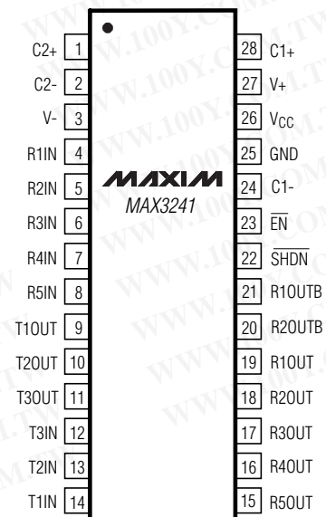
SO/SSOP/TSSOP
