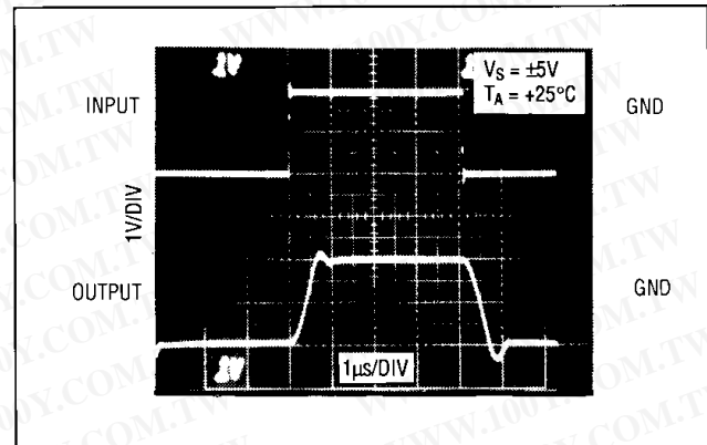
Figure 7b. Driving 680pF Load with 22Ω Isolation Resistor
