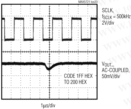
DIGITAL-TO-ANALOG GLITCH IMPULSE ( V_{DD} = +3\text{V} )
