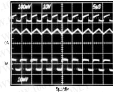
CONTINUOUS CONDUCTION AT FULL CURRENT LIMIT
