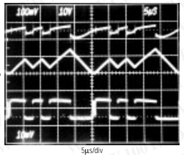
DISCONTINUOUS CONDUCTION AT HALF AND FULL CURRENT LIMIT
