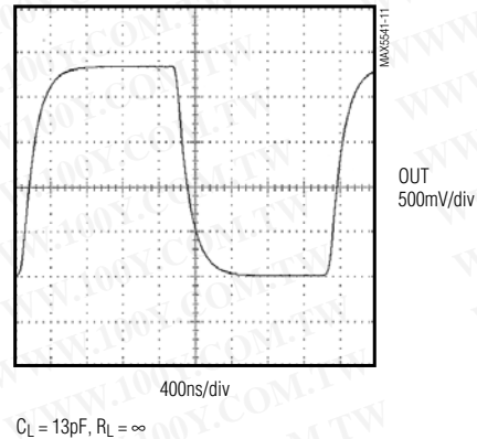
FULL-SCALE STEP RESPONSE ( f_{SCLK} = 20MHz )
