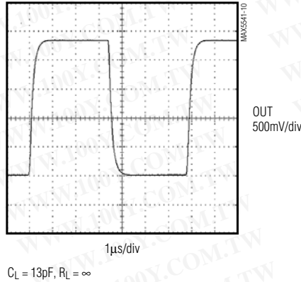
FULL-SCALE STEP RESPONSE ( f_{SCLK} = 10MHz )
