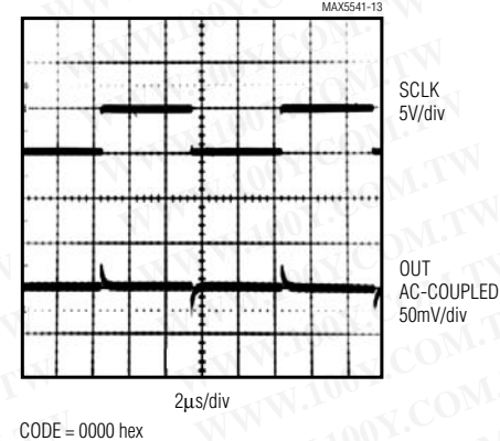
DIGITAL FEEDTHROUGH
