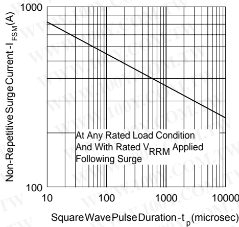
Fig. 7 - Max. Non-Repitative Surge Current
