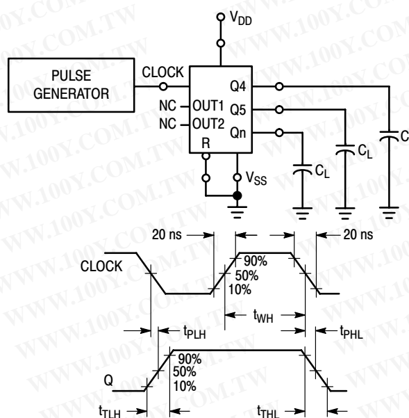
Figure 2. Switching Time Test Circuit and Waveforms
