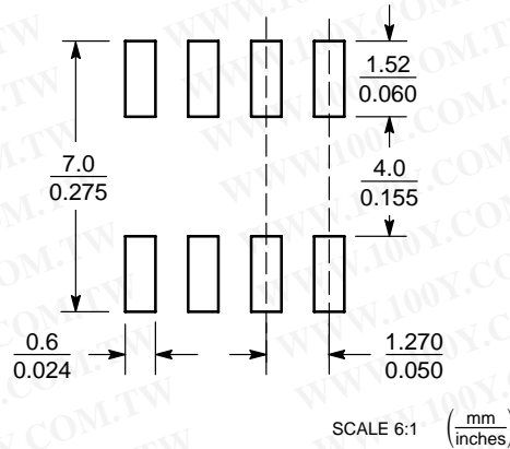
Figure 16. SO-8
