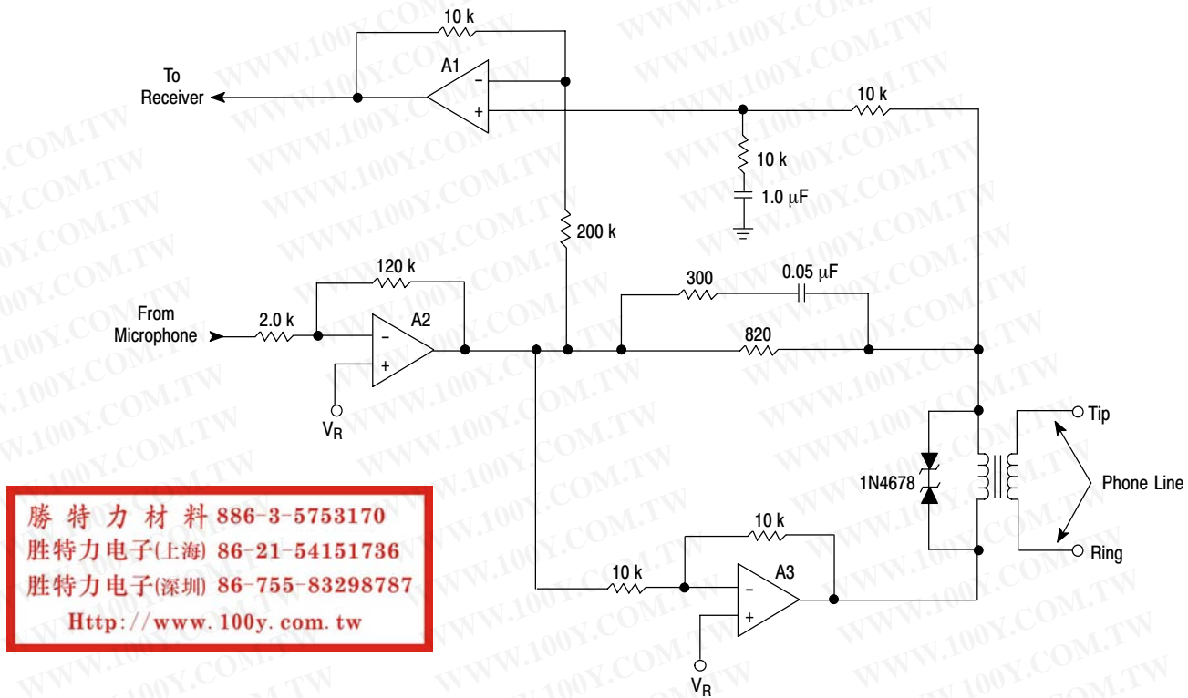
Figure 34. Telephone Line Interface Circuit
