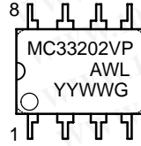
PDIP-8 VP SUFFIX CASE 626
