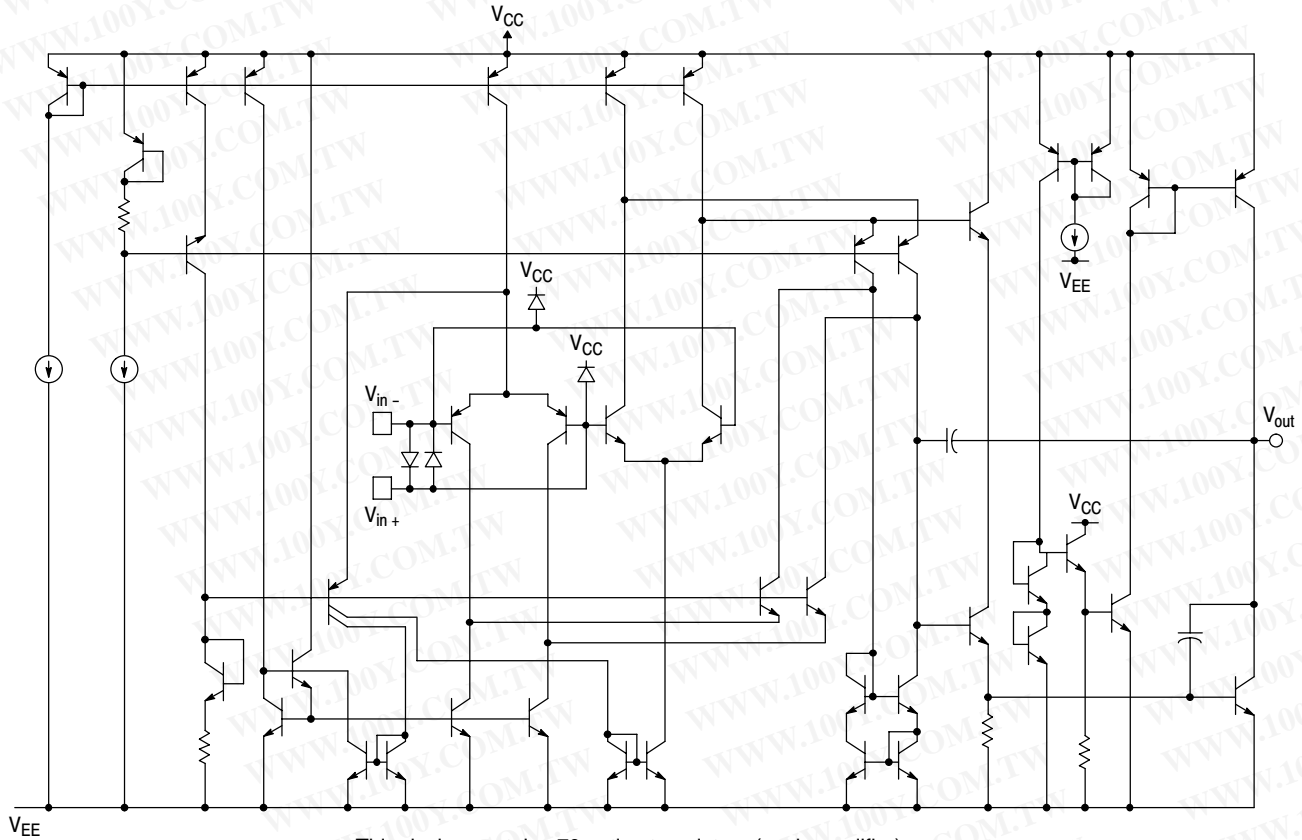
This device contains 70 active transistors (each amplifier).
