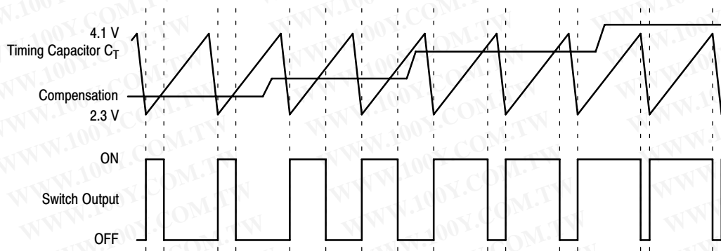
Figure 15. Timing Diagram
