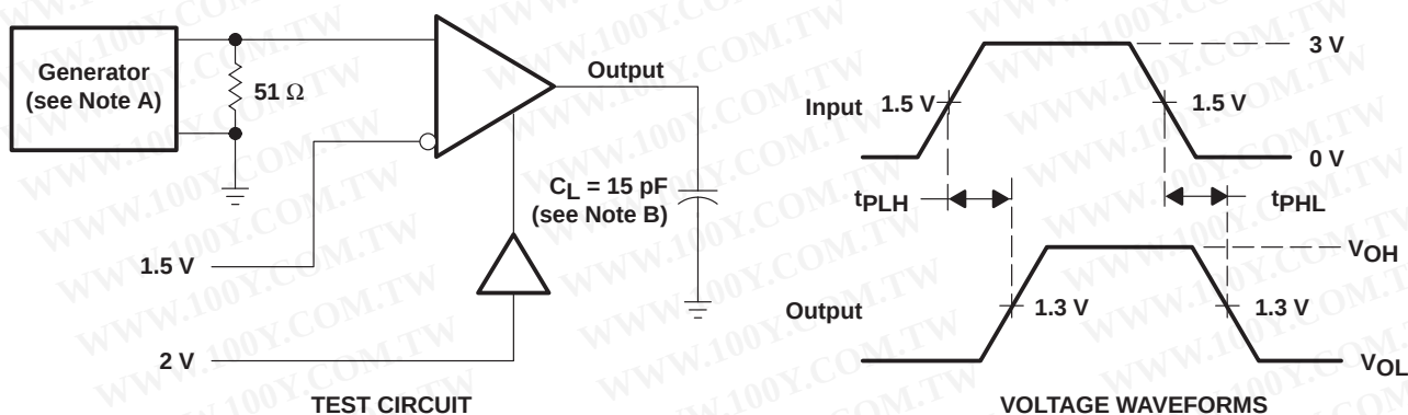
Figure 1. V_{OH} , V_{OL}
