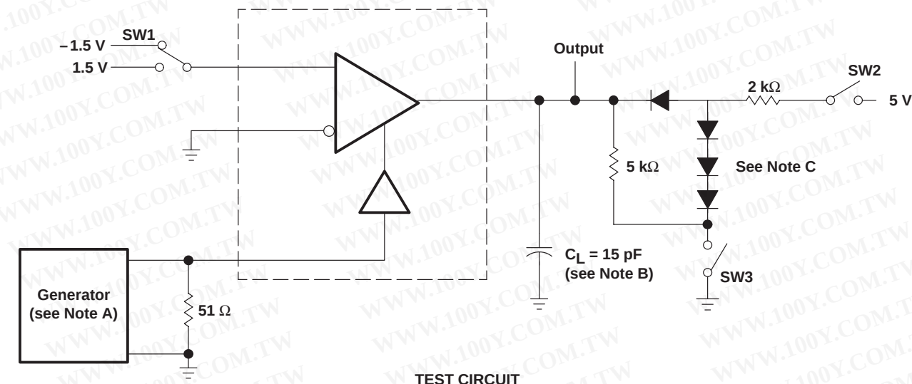
TEST CIRCUIT
