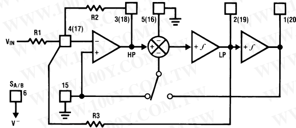
FIGURE 14. MODE 6a
