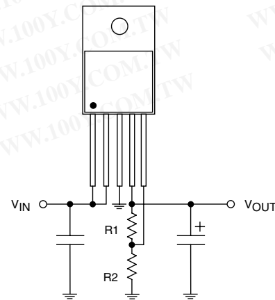
Figure 2. Adjustable Output Voltage Configuration. For best results, the total series resistance should be small enough to pass the minimum regulator load current.
