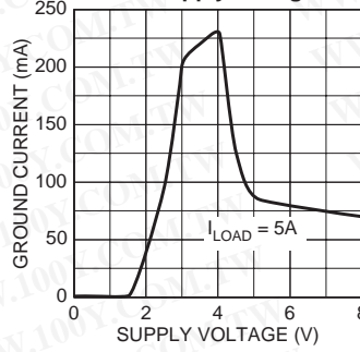
MIC2951x-3.3 Ground Current vs. Supply Voltage
