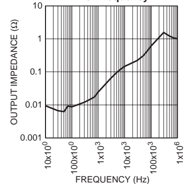
MIC2951x Output Impedance vs. Frequency
