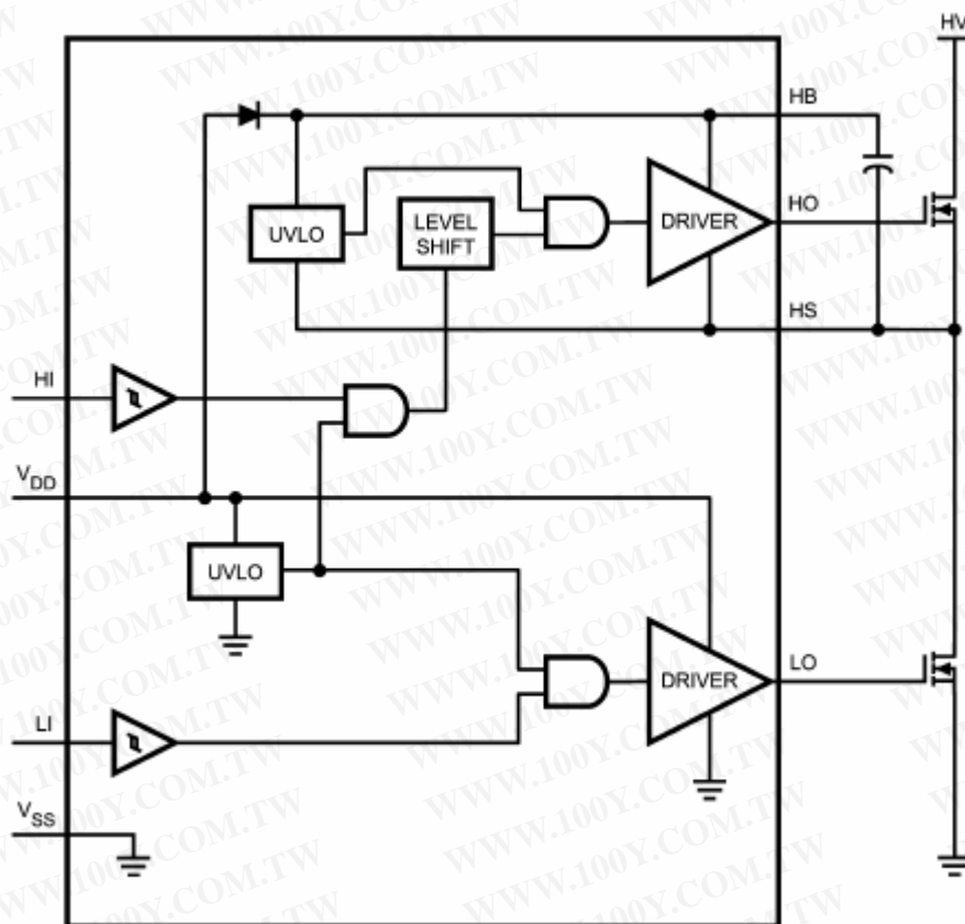
Figure 1. MIC4100 Functional Block Diagram
