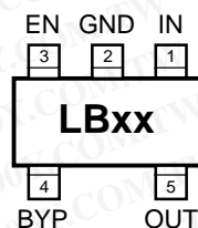
MIC5205-x.xBM5 Fixed Voltages
