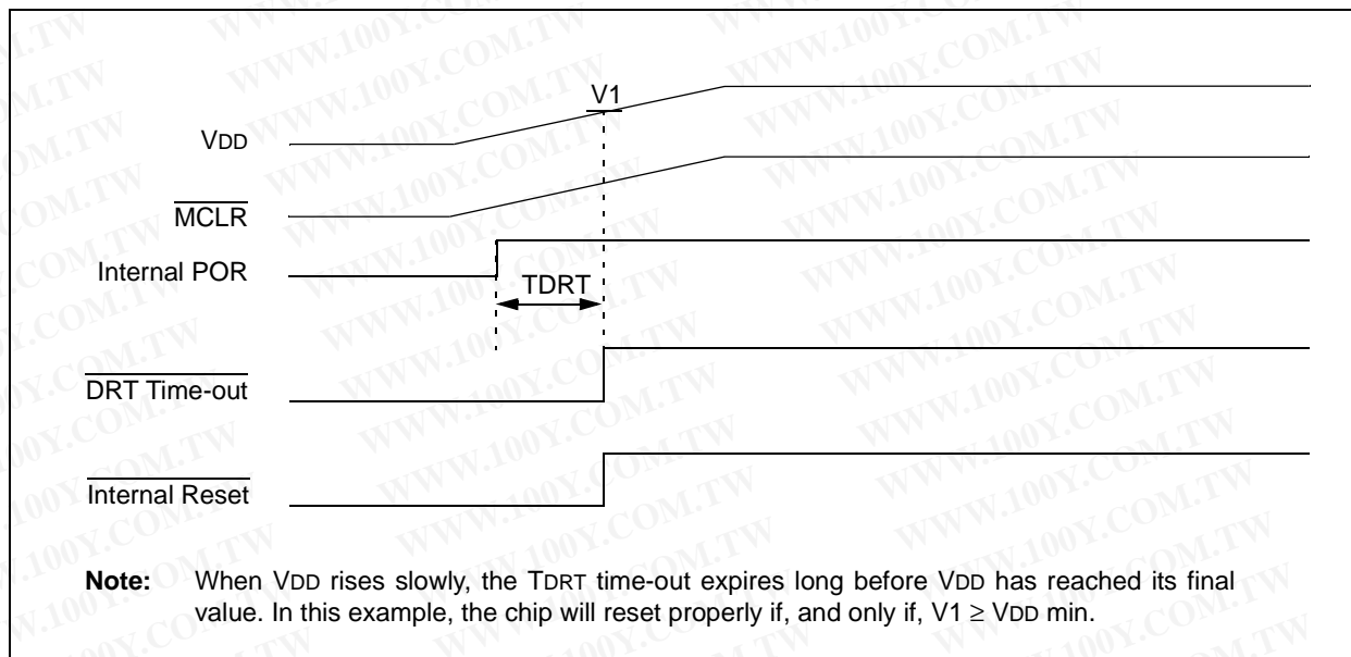
FIGURE 7-11: TIME-OUT SEQUENCE ON POWER-UP ( \overline{\text{MCLR}} TIED TO \text{V}_{\text{DD}} ): SLOW \text{V}_{\text{DD}} RISE TIME
