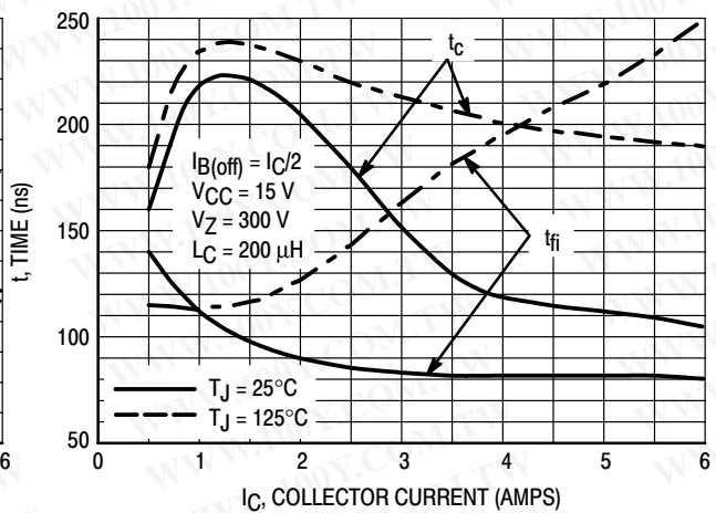
Figure 12. Inductive Switching, t_c and t_{fj} I_C/I_B = 10
