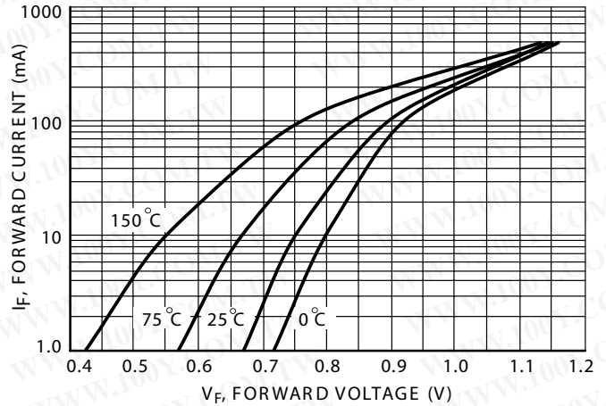
FIG.2 Typical Forward Voltage
