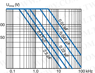
MMK7.5 ... 37.5 630/220
