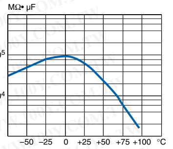
Insulation resistance vs. temperature
