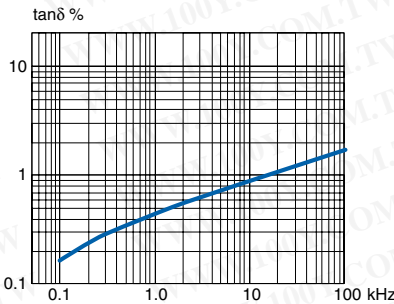
Dissipation factor vs. frequency (at +23°C)
