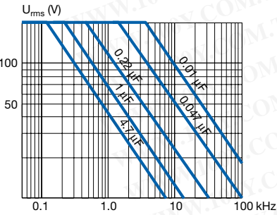
MMK7.5 ... 37.5 400/200
