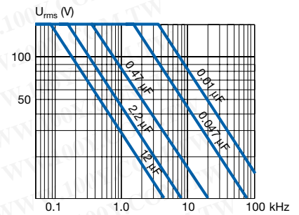
MMK7.5 ... 37.5 250/160
