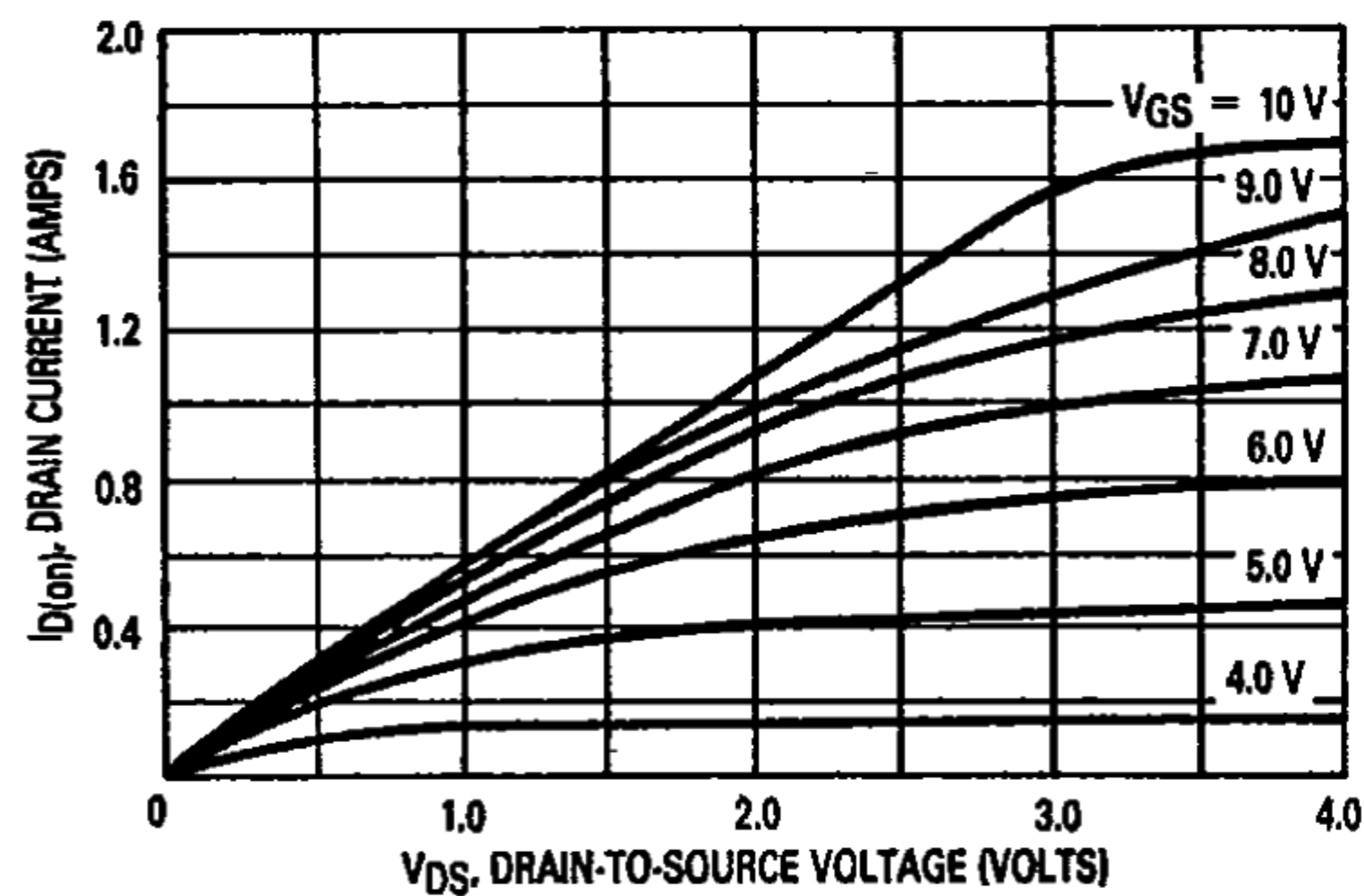
FIGURE 4 — ON-REGION CHARACTERISTICS
