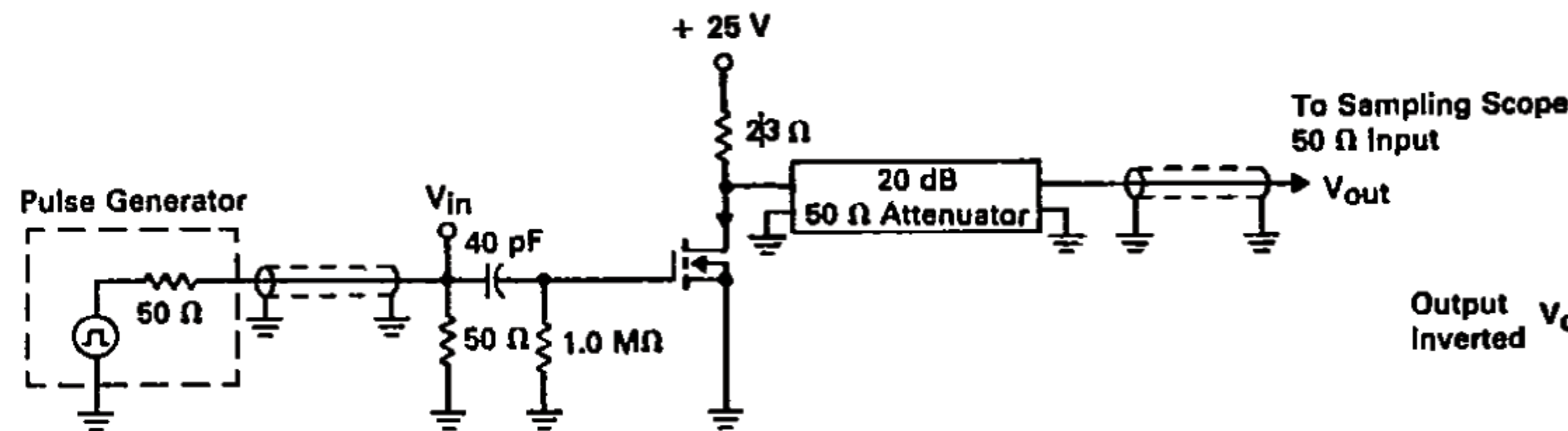
FIGURE 1 — SWITCHING TEST CIRCUIT
