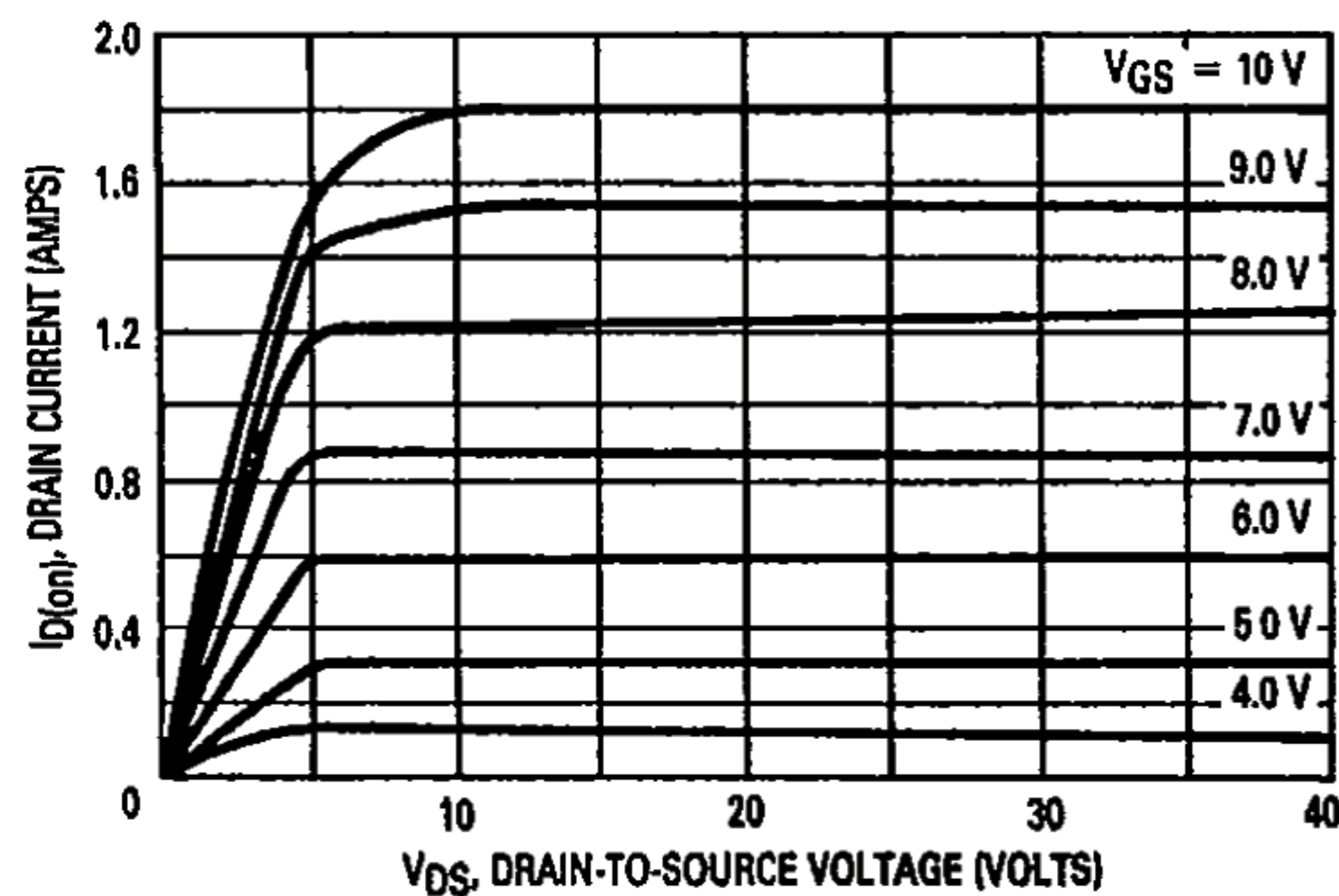
FIGURE 5 — OUTPUT CHARACTERISTICS
