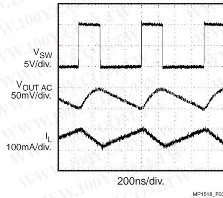
Figure 3—Steady State Operation
