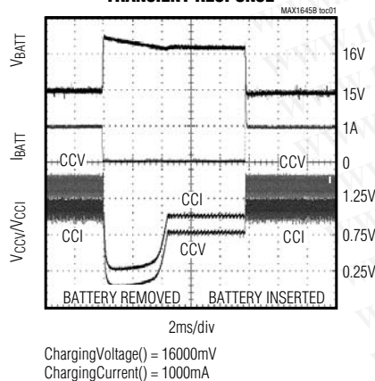
BATTERY REMOVAL AND REINSERTION TRANSIENT RESPONSE
