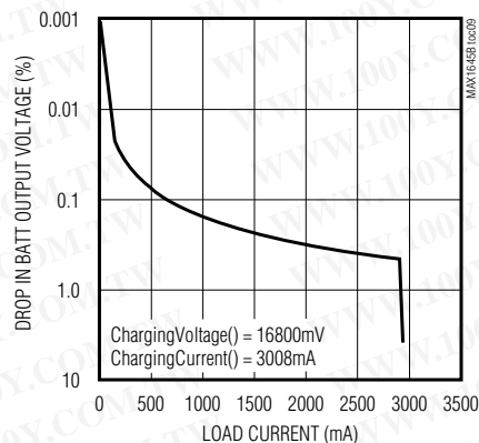
OUTPUT VI CHARACTERISTICS
