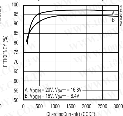
EFFICIENCY vs. BATTERY CURRENT (CURRENT-CONTROL LOOP)
