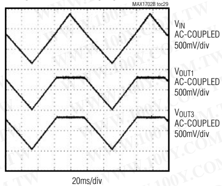
ENTERING AND EXITING DROPOUT WAVEFORM V_{IN} = 2.75\text{V TO } 4\text{V} , I_{LOAD1} = 250\text{mA} , I_{LOAD2} = 100\text{mA} , I_{LOAD3} = 200\text{mA}
