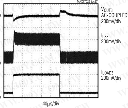
REG3 LOAD TRANSIENT WAVEFORM LOAD = 75mA TO 400mA, V_{IN} = 4\text{V}
