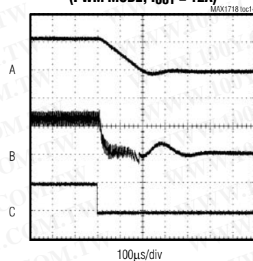
SHUTDOWN WAVEFORM (PWM MODE, I_{OUT} = 12A )
