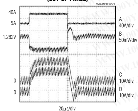
LOAD TRANSIENT (OUT-OF-PHASE)
