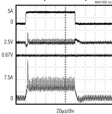
INDUCTOR SATURATION PROTECTION (LSAT DISABLED)
