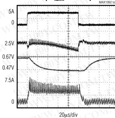
INDUCTOR SATURATION PROTECTION ( \Delta V_{LIM} = 200mV )
