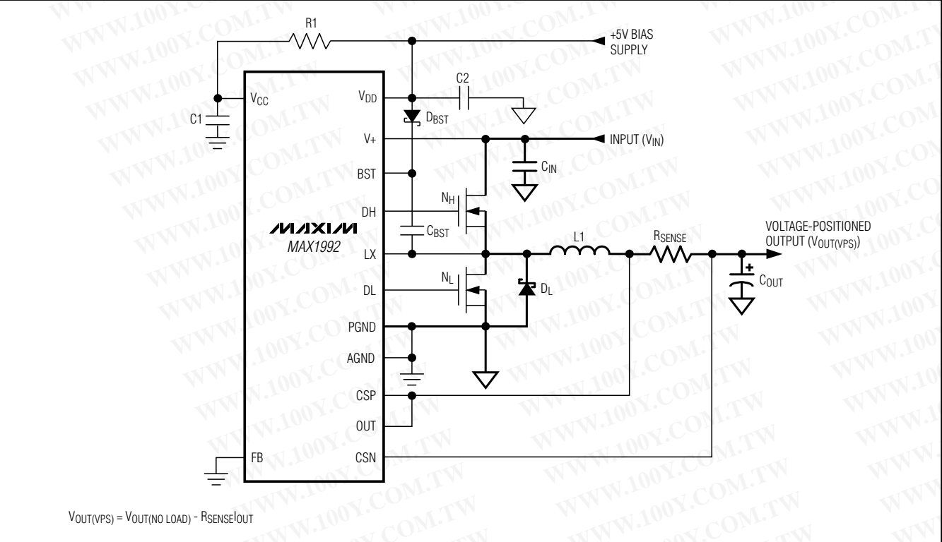
Figure 13. Voltage-Positioning Output
