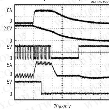
OUTPUT OVERLOAD WAVEFORMS (UVP ENABLED)
