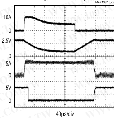
OUTPUT OVERLOAD WAVEFORMS (UVP DISABLED)
