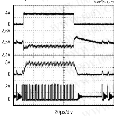
LOAD TRANSIENT (PULSE-SKIPPING OPERATION)
