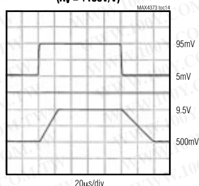
LARGE-SIGNAL PULSE RESPONSE ( A_V = +100V/V )
