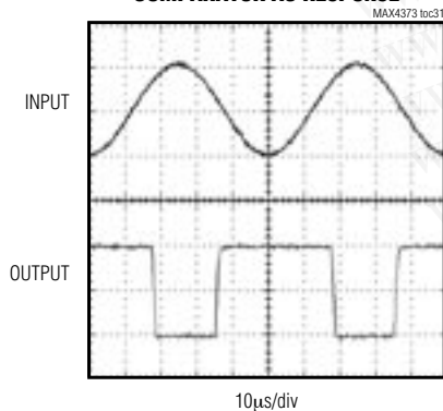
COMPARATOR AC RESPONSE
