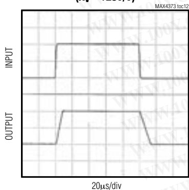
LARGE-SIGNAL PULSE RESPONSE ( A_V = +20V/V )
